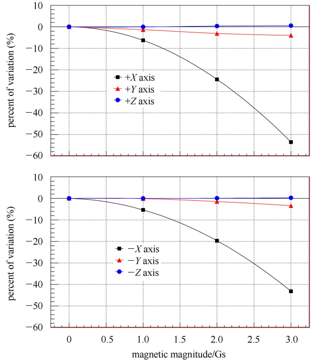
Fig. 5. PMT signal variation with the magnitude of magnetic field in \pm X , \pm Y and \pm Z directions.
