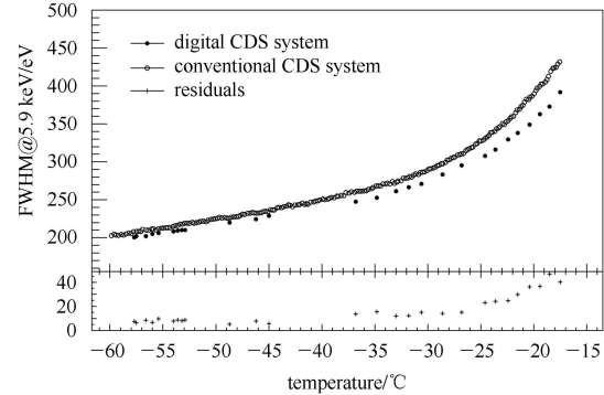
Fig. 11. Comparison of the energy resolution. The open circles, solid circles and plus signs ('+') represent the data of the conventional CDS system, the digital CDS system and the residuals, respectively.
