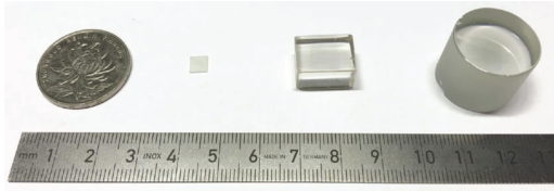
Fig. 2. CdMoO 4 crystals of different shapes, produced by Ningbo University.
