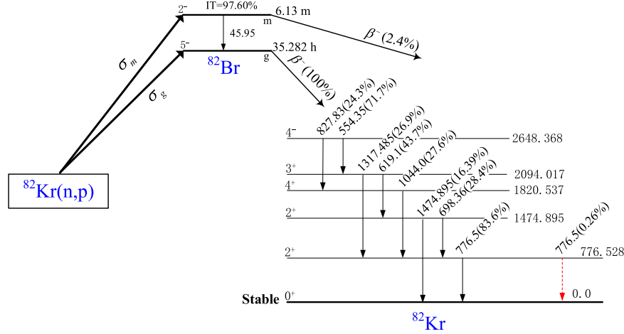
Fig. 1. (color online) The decay scheme of the radioactive nuclide ^{82\text{m}}\text{Br} [15], with the unit of energy in keV. The red dotted lines originate from the excited state, while the continuous black lines come from the ground state.
