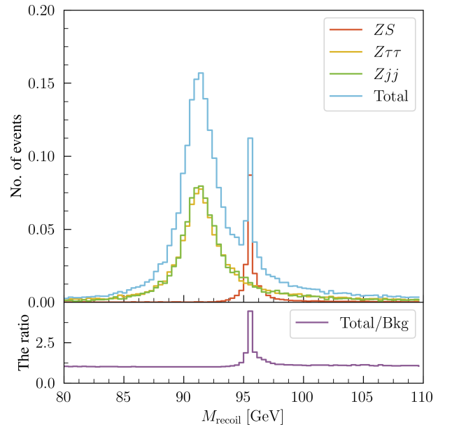
Fig. 1. (color online) Recoil mass distributions for the signal process ZS with M_S = 95.5 (normalized to 0.2), backgrounds Z\tau\tau and Zjj (normalized to 1), and the total (signal + background). The lower panel shows the ratio of the total to the background.
