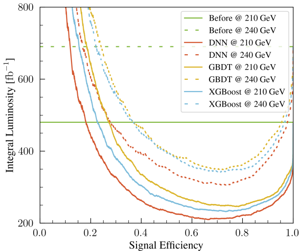
Fig. 3. (color online) Integrated luminosity required to reach 5\sigma significance at the benchmark point, as a function of the signal efficiency. Solid (dotted) curves correspond to \sqrt{s} = 210 (240) GeV. Colors denote different selection strategies: baseline (before applying ML classifiers, green), DNN (red), GBDT (yellow), and XGBoost (blue).
