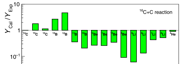
Fig. 11. (color online) Ratio of the calculated fragment yields to the measured ones, produced in ^{16}\text{C} + \text{C} reaction. The yield values are taken from Table 1.
