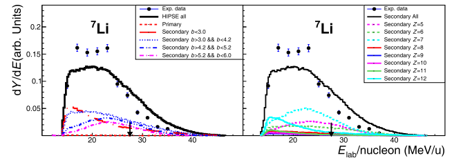
Fig. 10. (color online) Fragment-energy spectra for ^7\text{Li} produced in ^{16}\text{C} + \text{C} reaction (refer to Fig. 8 for the normalized presentation). Left panel: Experimental data with statistical error bars are compared with calculations characterized by secondary decay processes within different impact parameter ( b , in unit of fm) zones. Right panel: Calculated secondary decay processes characterized by mother nuclei which decay to ^7\text{Li} final fragment.
