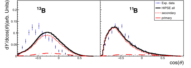
Fig. 9. (color online) Angular distributions of fragments ^{13}\text{B} and ^{11}\text{B} produced in ^{16}\text{C} + \text{C} reaction (refer to Fig. 8 for the normalized presentation). \theta is the azimuthal angle of the fragment defined in the beam-particle system and with the zero-degree axis pointing to the beam direction. Note that experimental or calculated fragments are filtered by the detection system. Error bars are statistical only. Panels in the same row share the same label inset.
