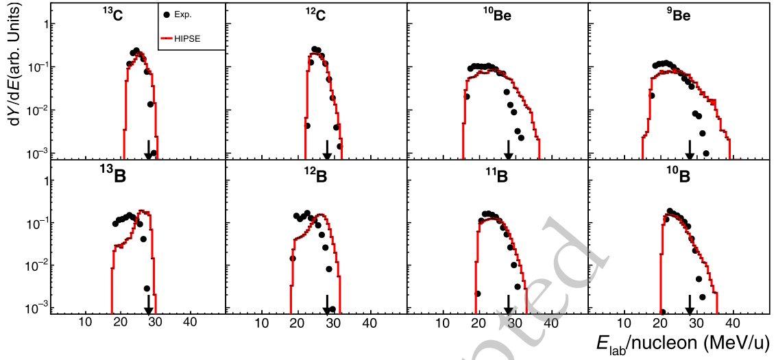
Fig. 4. (color online) Similar to Fig. 3 but for ^{14}\text{C} + \text{C} reaction at 27.5 MeV/nucleon.
