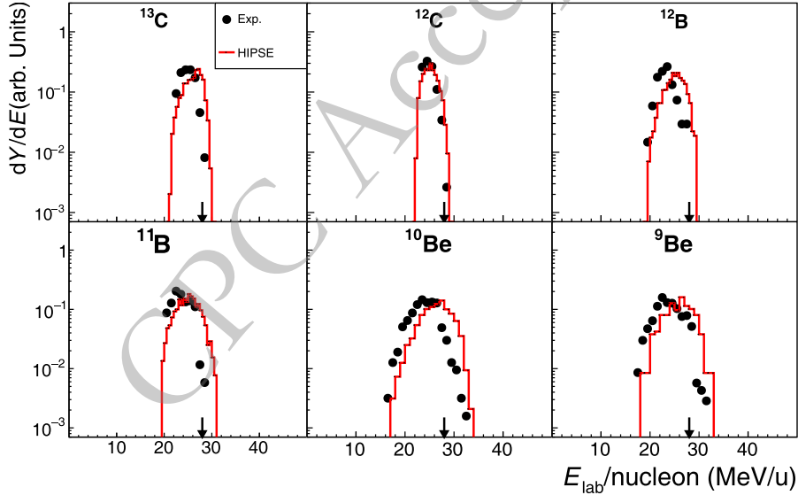
Fig. 7. (color online) Similar to Fig. 3 but for ^{14}\text{C} + d reaction at 27.5 MeV/nucleon.
