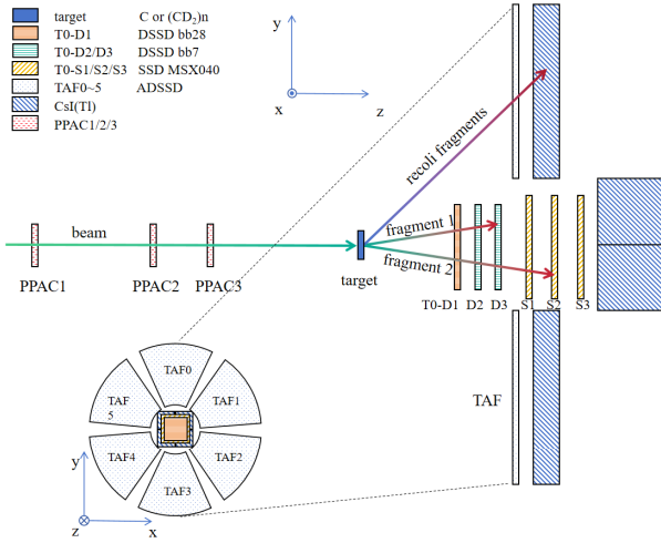
Fig. 1. (color online) Schematic view of the experimental setup. The beam is tracked by PPACs onto the target. Reaction fragments are detected by the T0 telescope, consisting of DSSDs and SSDs, and the surrounding TAF array. See texts for details.
