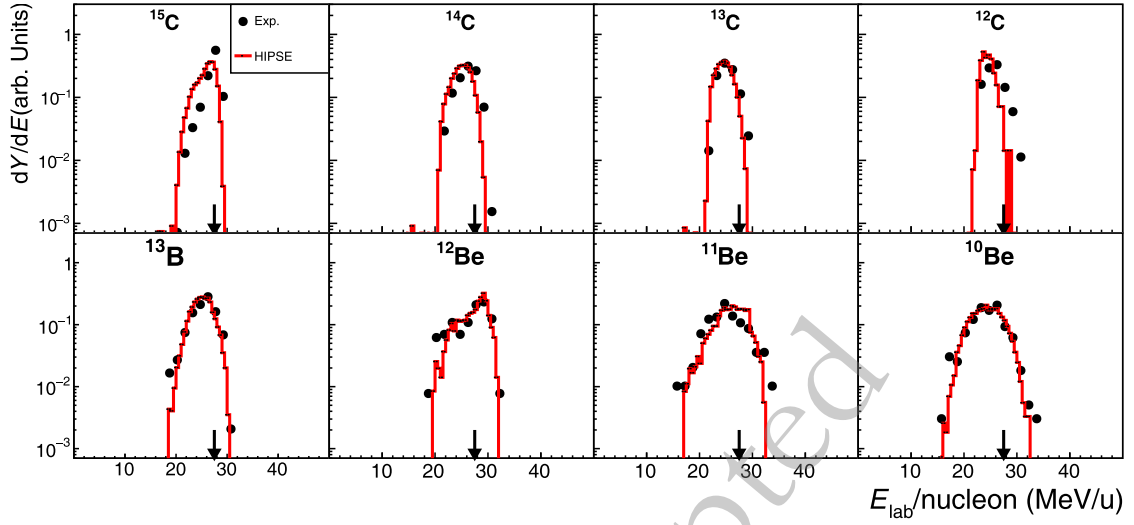
Fig. 6. (color online) Similar to Fig. 3 but for ^{16}\text{C} + d reaction at 27.5 MeV/nucleon.
