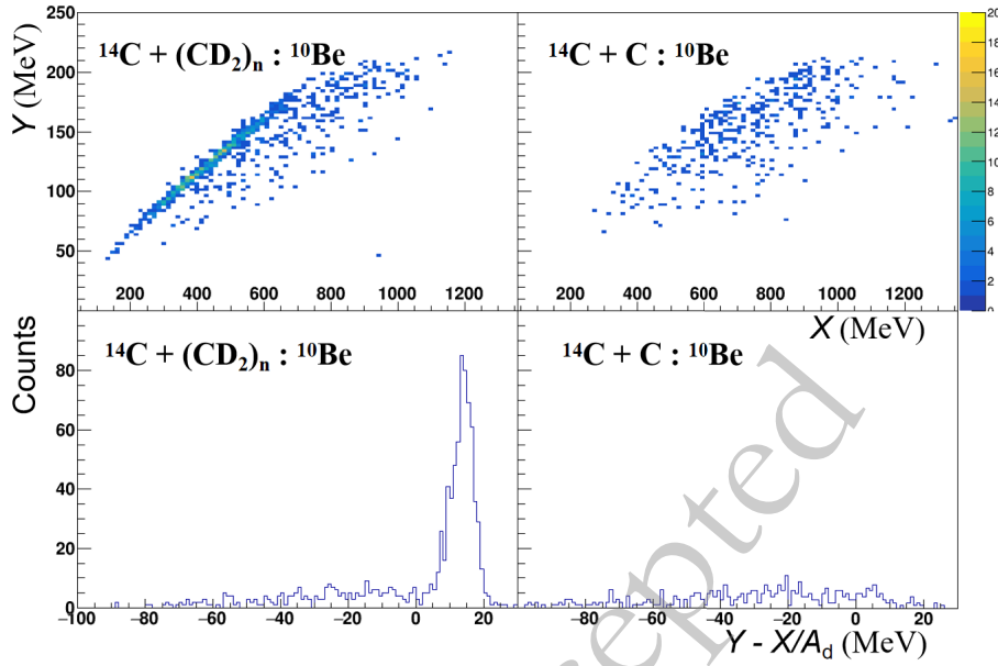
Fig. 5. (color online) An example of applying the extended E-P plot method, using data for coincidentally measured ^{10}\text{Be} fragment and recoil deuteron, produced in the reaction induced by ^{14}\text{C} beam at 27.5 MeV/nucleon on (\text{CD}_2)_n and carbon targets. The upper two panels show two-dimensional spectra for Y versus X , while the lower two panels present their projections, respectively, along the direction of the 1/A_d slope. X , Y and A_d are defined in Eq.2.
