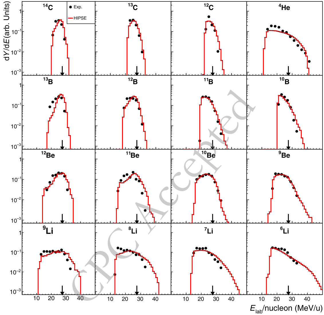
Fig. 3. (color online) Experimental Energy spectra (black-solid points) in comparison to the corresponding HIPSE-SIMON model calculations (red-solid lines) for fragments produced in the reaction ^{16}\text{C} + \text{C} at 27.5 MeV/nucleon [30, 33]. Each spectrum is normalized to its integral for a better shape comparison. The arrow in each panel indicates the incident beam energy per nucleon ( E_{\text{beam}}/\text{nucleon} ). The fragment (isotope) names are labeled in respective panels. The error bars are mostly small compared with the data-point size in the current logarithmic presentation and hence omitted in the figure.
