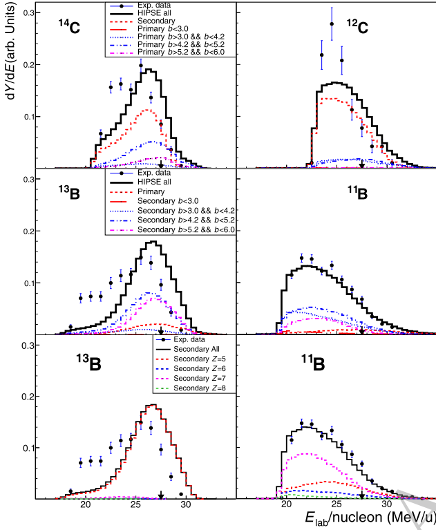
Fig. 8. (color online) Fragment-energy spectra for selected isotopes produced in ^{16}\text{C} + \text{C} reaction. In each panel the calculated spectra are normalized to the integral of the “all” spectrum while data points are presented relative the data integral (Error bars are statistical only) [30, 33]. Top panels for ^{14}\text{C} and ^{12}\text{C} isotopes: Experimental data in comparison to HIPSE-SIMON model calculations characterized by primary reaction processes within different impact parameter ( b , in unit of fm) zones having the equal zone-area; Middle panels for ^{13}\text{B} and ^{11}\text{B} : The comparisons characterized by secondary decay processes within different impact parameter zones; Bottom panels for ^{13}\text{B} and ^{11}\text{B} : Calculated secondary decay processes characterized by mother nuclei which decay to the actual final fragment. Panels in the same row share the same label inset.
