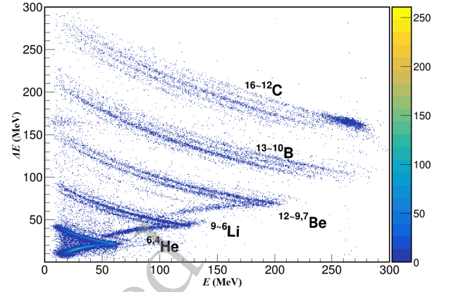
Fig. 2. (color online) Example of Particle identification (PID) spectra defined by the energy loss ( \Delta E ) and the remaining energy ( E ) as measured by T0-D1 and T0-D2 detectors, respectively, for the ^{16}\text{C} + \text{C} reaction at 27.5 MeV/nucleon. Each band corresponds to a specific isotope, demonstrating clear particle identification. For each element, mass numbers of the isotopes are labeled, with the higher number corresponding to the upper band.
