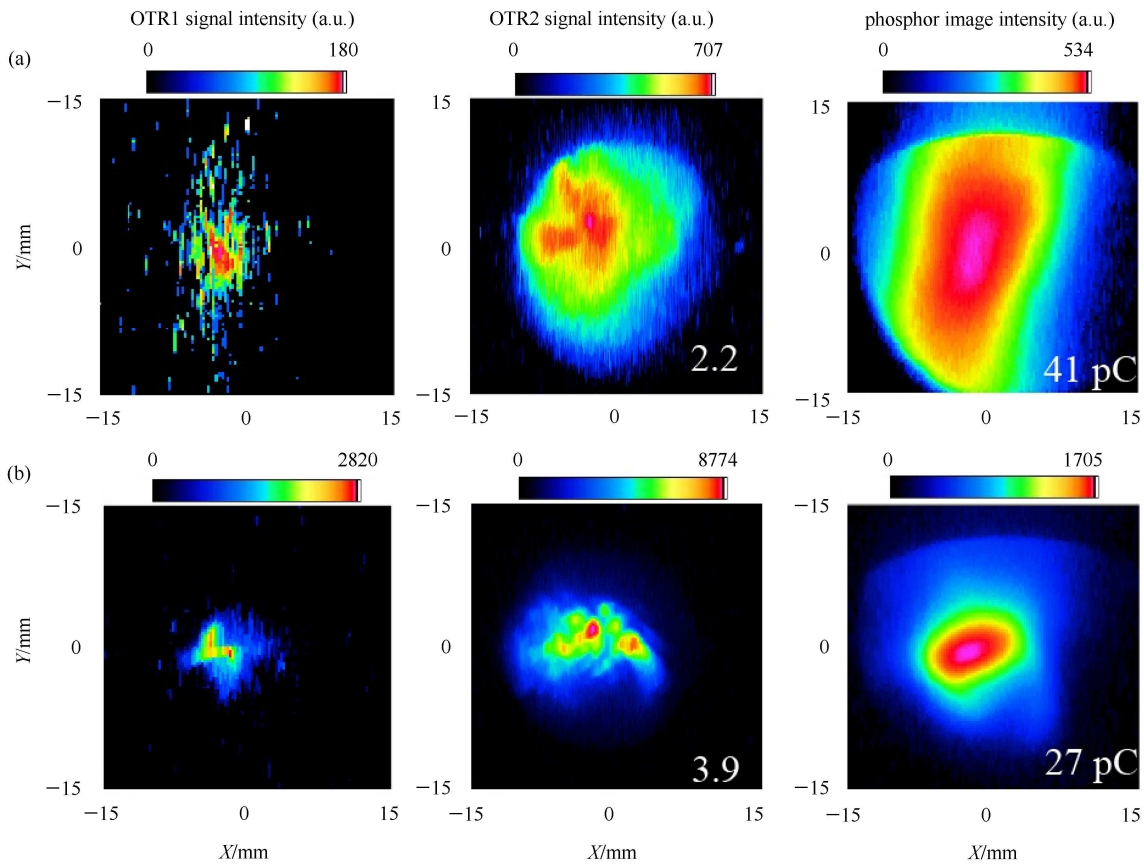
Fig. 4. The simultaneously taken single shot electron OTR1, OTR2 and phosphor near-field images, under the conditions of (a) without and (b) with the quadruples focusing. In OTR image, the white number is the coherent enhancement calculated based on the whole electron bunch charge. The beam charge information is also shown inside the phosphor image.
